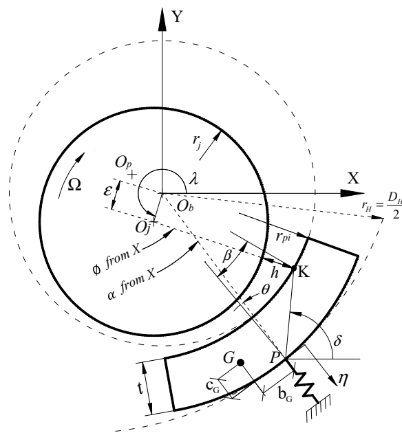
Figure 1. Detailed geometry of a pad of a rocker-backed TPJB [36].
