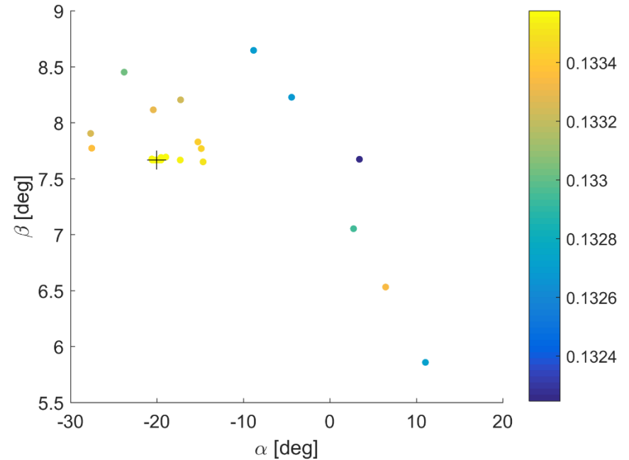
Deflection manoeuvre
