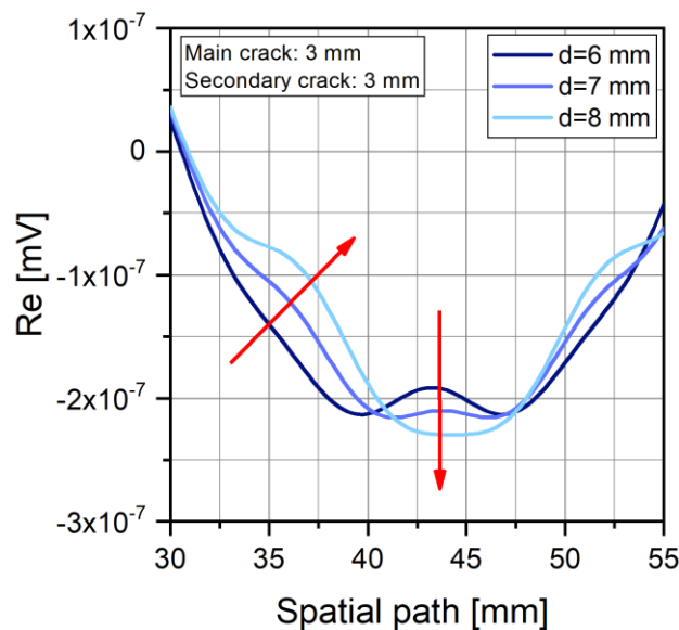
Figure 8: Quantification of the spatial resolution of the prototype.
