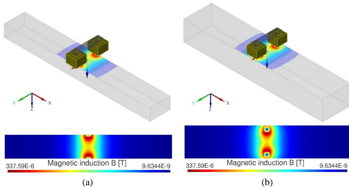
Figure 4: Field of action of the customized probe in terms of magnetic induction: a) case of the smallest tie-rod in the Milan cathedral; b) case of the largest tie-rod in the Milan cathedral.
