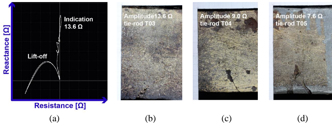
Figure 10: a) Impedance plane at defect on T03; defect on b) T03, c) T04 and d) T05
