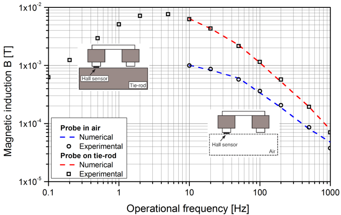
Figure 3: Validation of the numerical model by experimental acquisitions of magnetic induction on T01 tie-rod.
