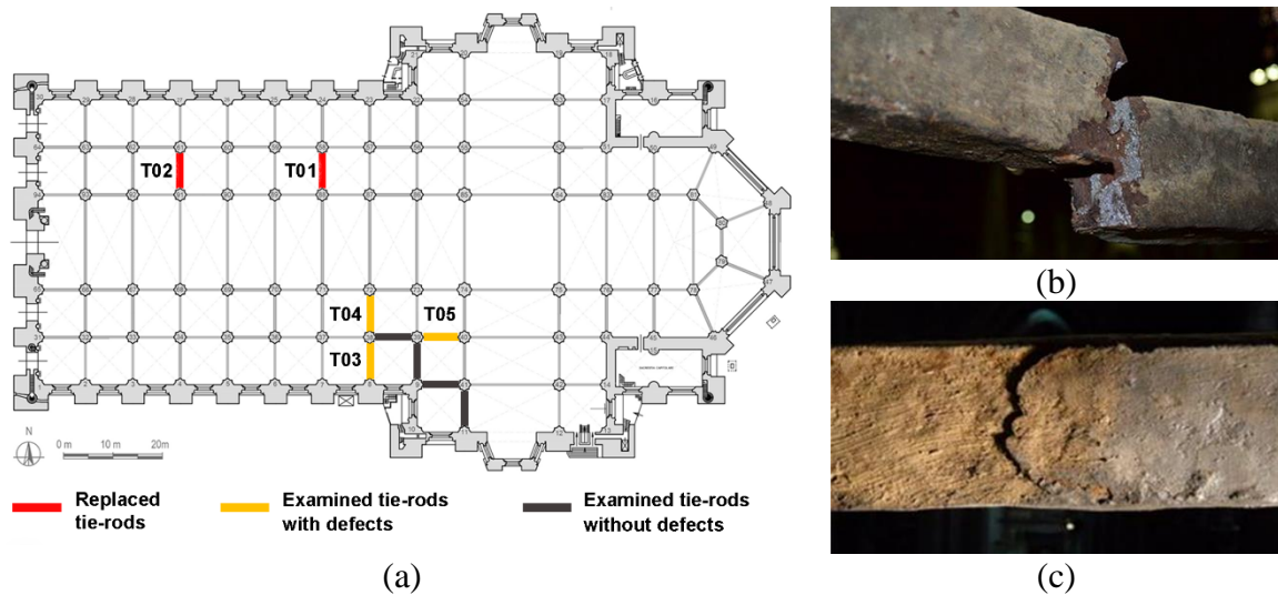
Figure 1: Milan cathedral: a) scheme of the location of tie-rods discussed in this paper; Failed tie-rods: b) broken in two parts, T01; c) with a visible crack, T02
