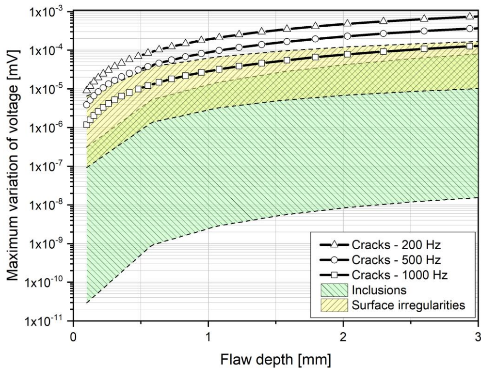
Figure 5: Numerical sensitivity analysis, about the operative frequency, based on flaws of different nature, shape and dimensions.
