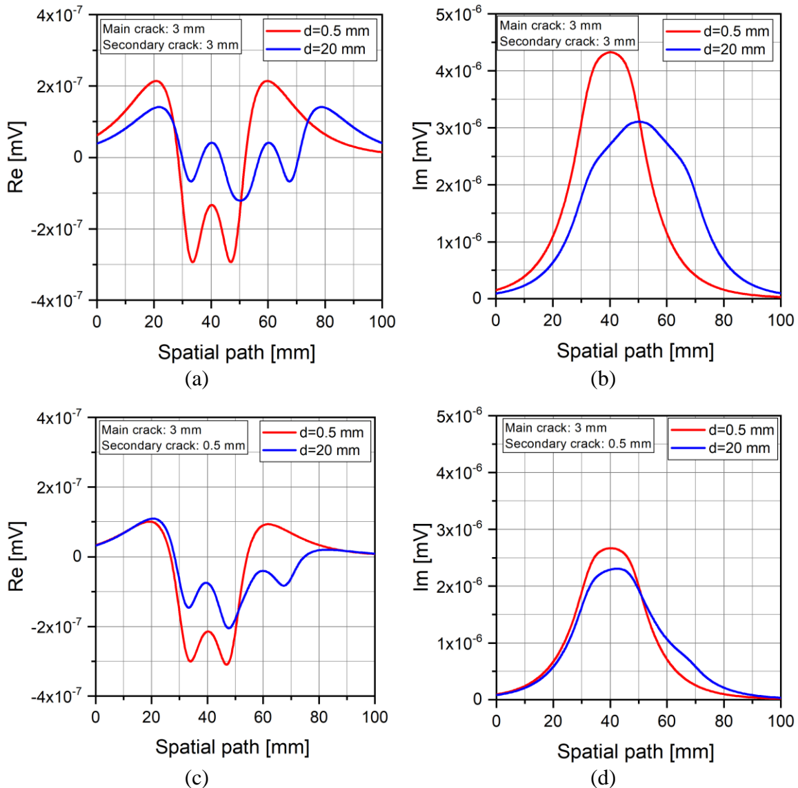
Figure 7: Analysis of the real and imaginary parts of the maximum variation of voltage through the coils in terms of the instantaneous position of the probe during the simulated inspection.
