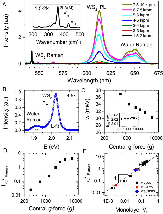
Figure 5: Photoluminescence data for dispersions with different monolayer content. A) Photoluminescence ( \sim 610 nm) and Raman ( \sim 540 nm) spectra of surfactant-stabilized WS 2 dispersions prepared with different centrifugation conditions and measured in liquid using a Raman spectrometer ( \lambda_{exc}=532 nm). The spectra were normalized to the 2LA(M) Raman mode of WS 2 . The feature at \sim 650 nm is the water Raman peak. Inset: Raman spectrum of dispersed WS 2 nanosheets plotted versus wavenumber. B) Photoluminescence spectrum of WS 2 , plotted on an energy scale and fitted to a Lorentzian. C) PL linewidth, from Lorentzian fit, plotted versus central centrifugation acceleration (expressed in units of g ). Inset: PL position vs. g -force. D) Ratio of PL intensity to Raman intensity, I_{PL}/I_{Raman} , plotted vs. g -force. E) I_{PL}/I_{Raman} plotted versus monolayer volume fraction. The dashed line represents I_{PL}/I_{Raman} = 17 \times V_f .
