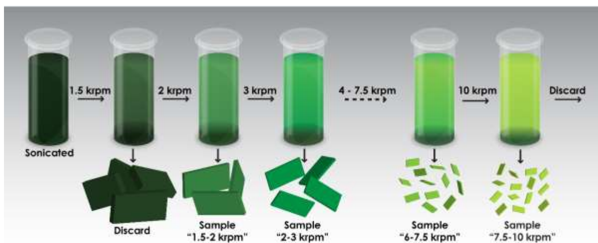
Figure 1: Schematic describing the basic centrifugation cascade employed in this study. The sediment discarded after the first centrifugation contains exfoliated layered crystallites while the supernatant discarded after the last centrifugation step contains extremely small nanosheets. Size-selected dispersions are prepared by re-dispersing the collected sediments in 1 g/L aqueous sodium cholate after subsequently increasing centrifugation speeds.
