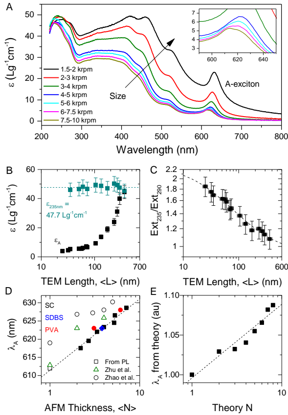
Figure 4: Dependence of the optical properties of nanosheet dispersions on the nanosheet dimensions. A) Optical extinction coefficient spectra measured for WS 2 dispersions (water/SC) prepared using different centrifugation conditions, and so with different mean nanosheet lengths and thicknesses. Inset: magnified A-exciton region. B) Extinction coefficient, measured at 235 nm and at the A-exciton position (~615nm) plotted versus mean nanosheet length, as measured by TEM. The mean value of \epsilon_{235\text{nm}} is 47.7 \text{ Lg}^{-1}\text{cm}^{-1} . C) Ratio of extinction at 235 nm to that at 290 nm plotted versus mean nanosheet length, as measured by TEM. The dashed line is a fit to eq. 2. D) A-exciton center of mass position (determined from second derivatives) plotted versus mean nanosheet thickness. Also included is data for WS 2 nanosheets dispersed in SDBS and PVA and from the literature. 51, 52 The open symbol represents the A-exciton position from photoluminescence measurements. The dashed line shows an empirical relationship between \lambda_A and N according to eq. 4. E) Calculated relative wavelength associated with the optical gap of WS 2 ( i.e. the direct band gap at the K-point).
