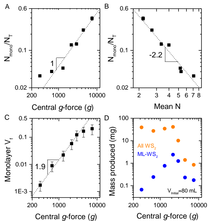
Figure 3: Monolayer population data extracted from histograms for a range of centrifugation conditions. A) Number fraction of monolayers, N_{\text{mono}}/N_{\text{T}} , as a function of the central centrifugation acceleration, presented as g -force. B) Plot of N_{\text{mono}}/N_{\text{T}} versus mean nanosheet thickness, N . C) Monolayer volume fraction as a function of g -force. D) Total mass of all \text{WS}_2 as well as only monolayer- \text{WS}_2 produced in each fraction as a function of g -force.
