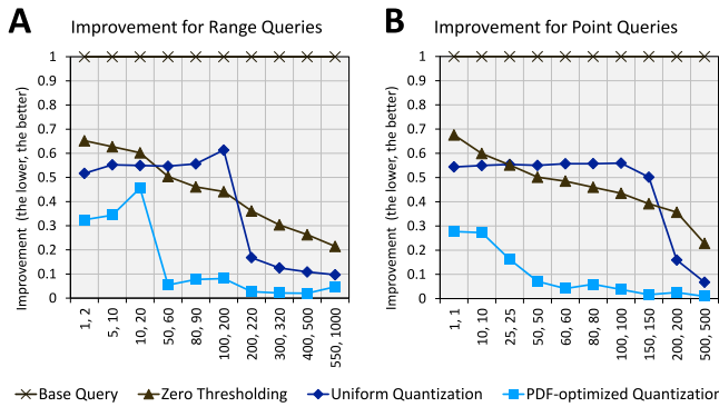
Fig. 8. Second resolution evaluations. Panels A and B the performance of the three built-in methods for secondary resolution normalized to base query time.
