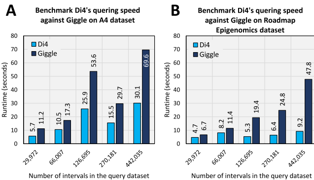
Fig. 7. The runtime plotted here is the average of 10 executions of each query. The results show that Di4 runs up to 3\times faster than Giggle on a large dataset (panel A), and up to 6\times faster on a small dataset (panel B).
