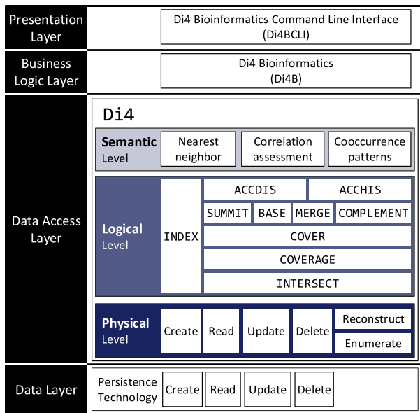
Fig. 1. Di4 architecture and functional components.
