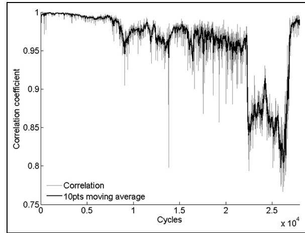
Figure 10. Correlation coefficient of Chebyshev moments of wavestream number 100 and all other wavestreams.
