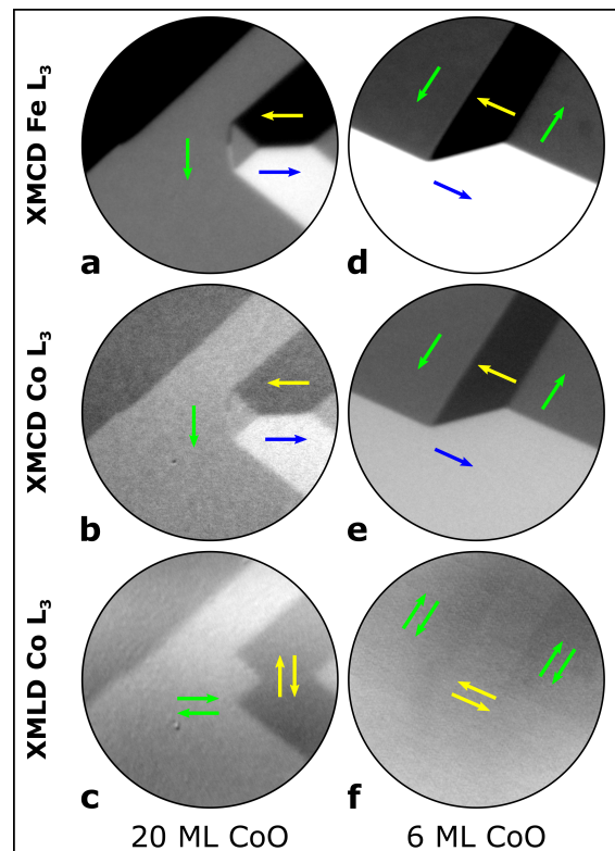
Figure 3: XMCD-PEEM and XMLD-PEEM images taken at the reported absorption edges for CoO/Co/Fe samples with CoO thickness t_{\text{CoO}} = 20\ \text{ML} (panels a-c) and t_{\text{CoO}} = 6\ \text{ML} (panels d-f). The field of view is 20\ \mu\text{m} in all cases.
