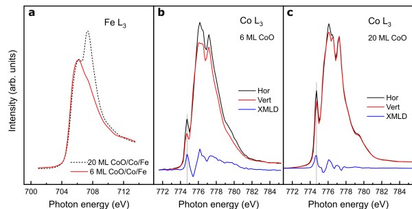
Figure 2: Panel a: XAS spectra at the Fe L_3 absorption edge on CoO/Co/Fe samples with different CoO thickness t_{\text{CoO}} (dashed black curve: t_{\text{CoO}} = 20 ML; continuous red curve t_{\text{CoO}} = 6 ML). Panels b and c: XAS spectra at the Co L_3 absorption edge for the same samples, taken with orthogonal linear polarizations (Hor, black line, in-plane polarization; Vert, red line, out-of-plane polarization) and XMLD spectra (blue curves) calculated from the corresponding XAS spectra.
