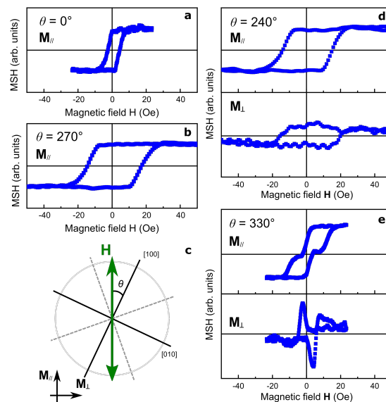
Figure 1: Panels a, b, d, e: magnetic second harmonic hysteresis loops on a 25 ML CoO film on Co/Fe(001). Panel c: sketch of the experimental layout. The parallel and perpendicular components of the in-plane magnetization \mathbf{M} are referred to \mathbf{H} .
