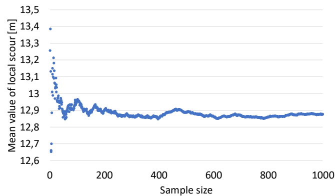
Figure 9. Bar chart of defuzzified values of local scour (top) and convergence curve of the related mean value (bottom).
