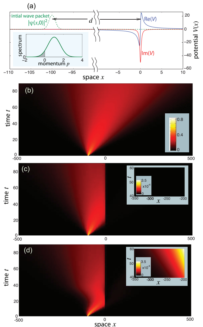
FIG. 3. (color online) Numerical simulations showing scattering of a wave-packet with broad momentum distribution from a single-pole dissipative Kramers Kronig potential [Eq.(34)] for parameter values V_0 = 10 and \alpha = 0.2 . (a) Behavior of the real and imaginary parts of V(x) (solid curves). To make the potential short-range, V(x) is enveloped by the broad super-Gaussian amplitude \exp[-(x/b)^4] with b = 60 . The initial wave-packet is \psi(x, 0) \propto \exp[-(x+d)/w^2 + ip_0 x] with d = 100 , w = 1.2 and p_0 = 1 . The dashed curve shows the initial wave-packet probability distribution |\psi(x, 0)|^2 , whereas the inset on the left bottom depicts the momentum distribution of the wave-packet. Note that negative momentum components are non-negligible. (b) Free evolution of the wave-packet \psi^{(free)}(x, t) in the absence of the external force and of the scattering potential, i.e. for F = V = 0 [snapshot of \sqrt{|\psi(x, t)|} on a pseudo color map]. (c) Same as (b), but with the scattering potential V(x) and without the external force ( F = 0 ). (d) Same as (b), but when the wave-packet is accelerated by the force given by Eq.(35) with parameter values T = 40 and F_0 = 0.25 . The insets in (c) and (d) show the behavior of |\psi^{(free)}(x, t) - \psi(x, t) \exp(i\phi_0)| in the upper-left region of space-time (x, t) , far from the scattering region and at times after switching off the external force.
