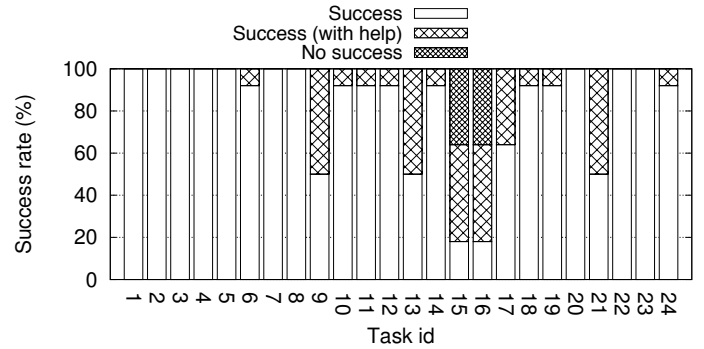
Figure 8. Success rates per modeling task.
