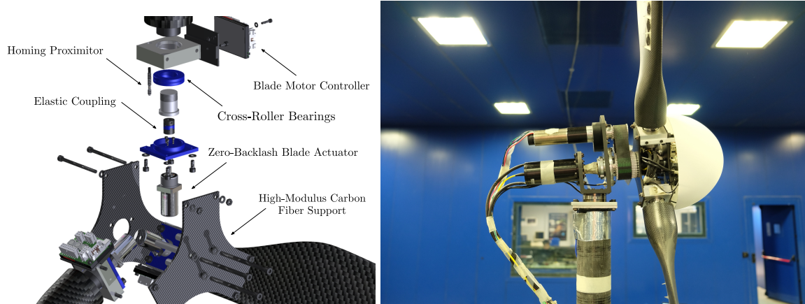
Fig. 7. Rotor exploded view (left) and assembly (right)
