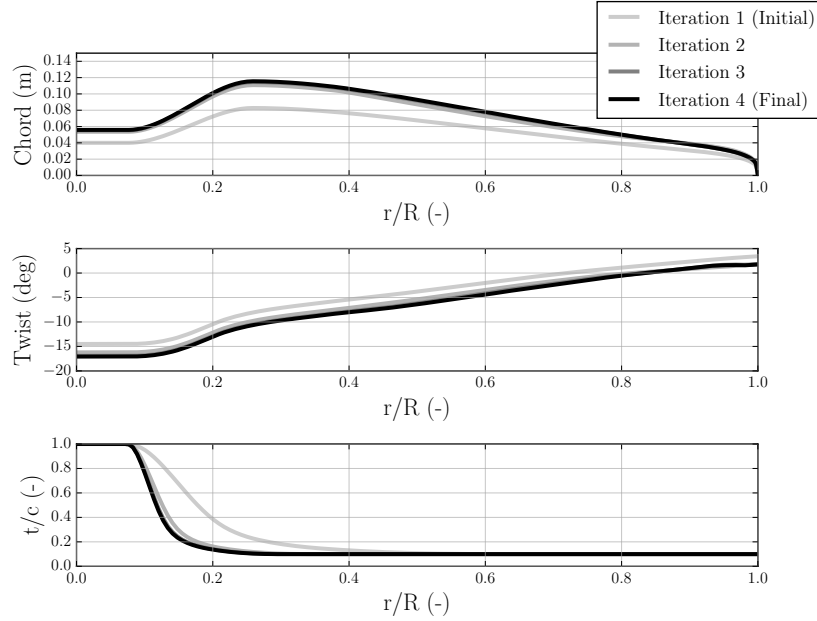
Fig. 4. Blade design iterations
