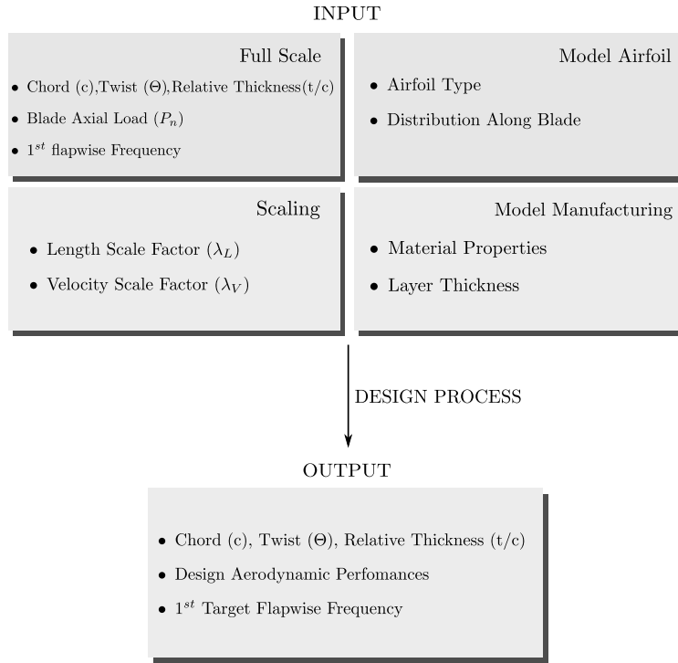
Fig. 1. Aerodynamic design scheme
