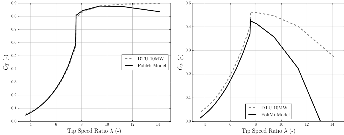
Fig. 5. Model Vs Full Scale performance (numerical computations): Power Coefficient C_T (left), Thrust Coefficient C_P (right).
