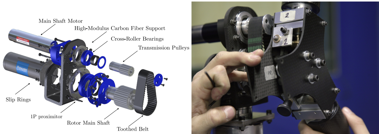
Fig. 6. Nacelle exploded view (left) and assembly (right)
