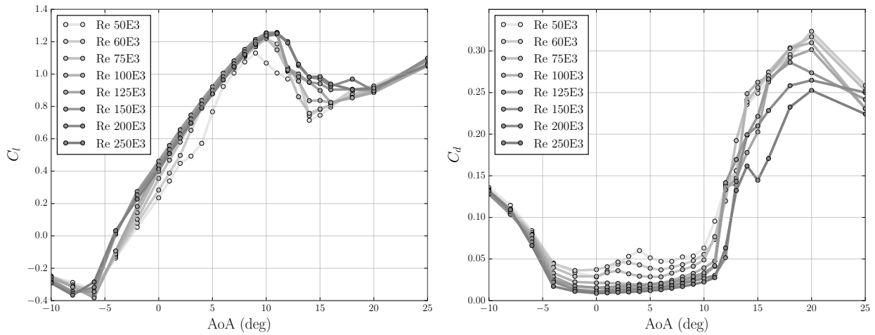
Fig. 3. Experimental aerodynamic coefficients: Lift coefficient C_l from pressure measurements (left), Drag coefficient C_d from force measurements (right)
