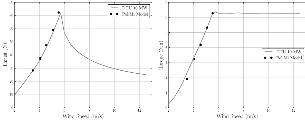
Fig. 9. Wind tunnel test results, for \lambda_V = 2 : thrust (left) and torque (right)
