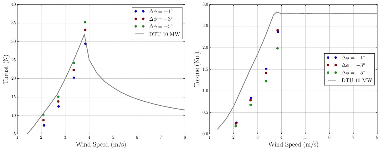
Fig. 10. Wind tunnel test results, for \lambda_V = 3 : thrust (left) and torque (right), for different variation of the blade pitch angle ( \Delta\phi ) with respect to the full scale nominal value.
