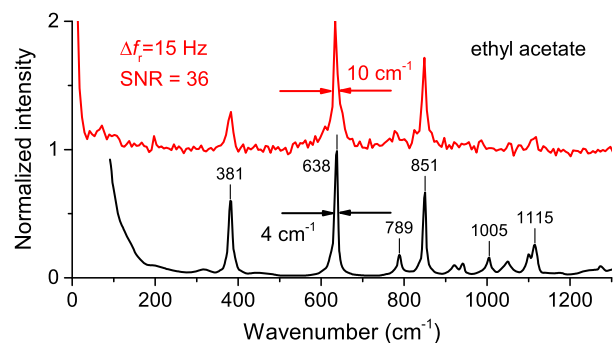
Fig. 6. Dual-comb CARS spectrum of ethyl acetate (red line), as calculated by Fourier transform of a single-windowed interferogram (30 \mu\text{s} observation time) and reference Raman spectrum of pure ethyl acetate [15].
