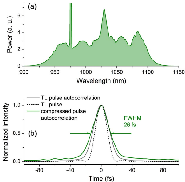
Fig. 3. (a) Spectrum of the supercontinuum radiation generated by the PCF fiber; the peak at 980 \text{ nm} is due to residual pump power. (b) Autocorrelation trace of compressed pulses as measured after the SF10 prism pair (green line) and of transform-limited pulses (gray line). The transform-limited pulses of 17\text{-fs} duration are also represented (dotted line).
