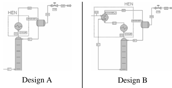
Fig. 1: project design solutions compared in steady and unsteady analysis.
