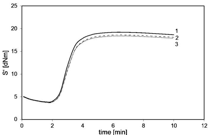
FIG. 17. — Rheometric curves obtained at 170 °C for composites of Table II containing different amounts of CB–SP: (1) 0 phr; (2) 5 phr; (3) 7.5 phr.
