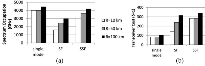
Fig. 4. Spectrum occupation and transceiver cost obtained when minimizing S_o with one-to-all traffic matrix and 10 Tb/s overall traffic, assuming \delta = 1 . (a) Minimization of S_o , (b) C_t when minimizing S_o .
