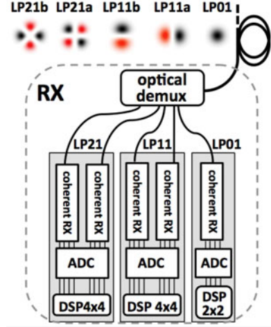
Fig. 3. The considered receiver model.
