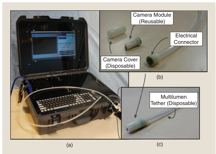
Figure 2. (a) The HydroJet platform designed to be easily transportable, (b) the HydroJet capsule disassembled into disposable and reusable components, and (c) the HydroJet capsule.
