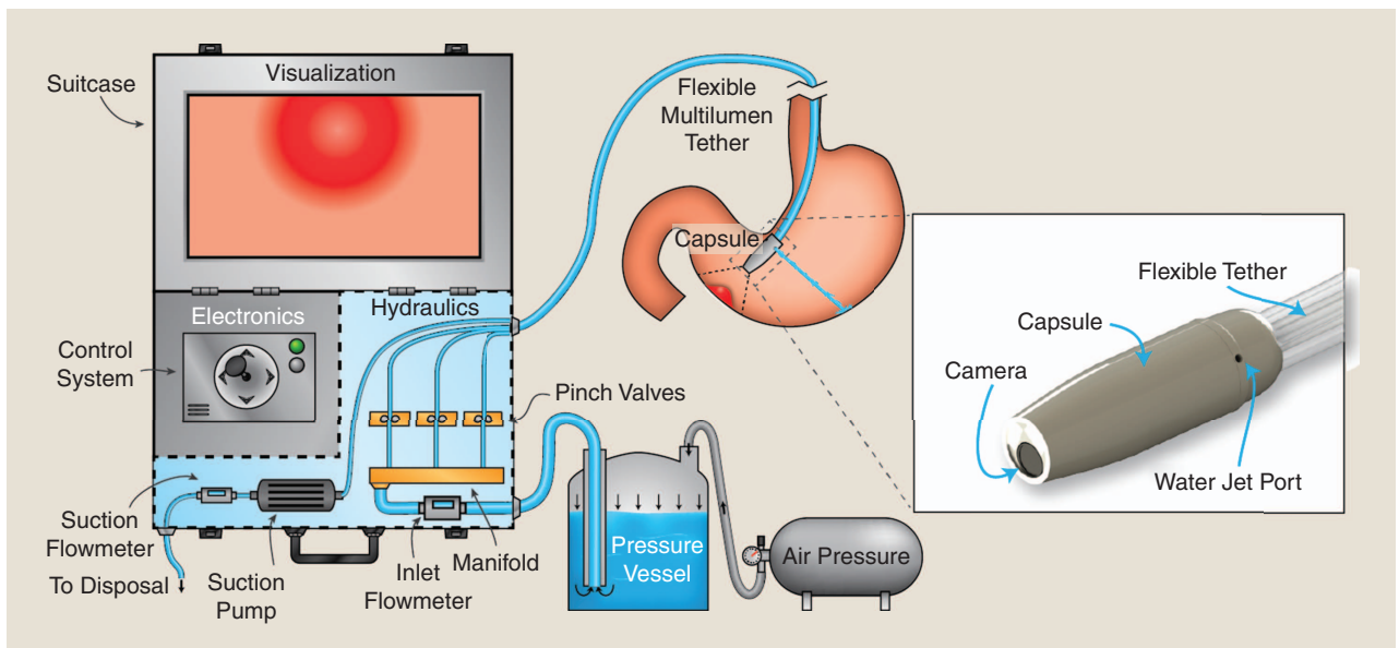
Figure 1. A diagram of the HydroJet system.
