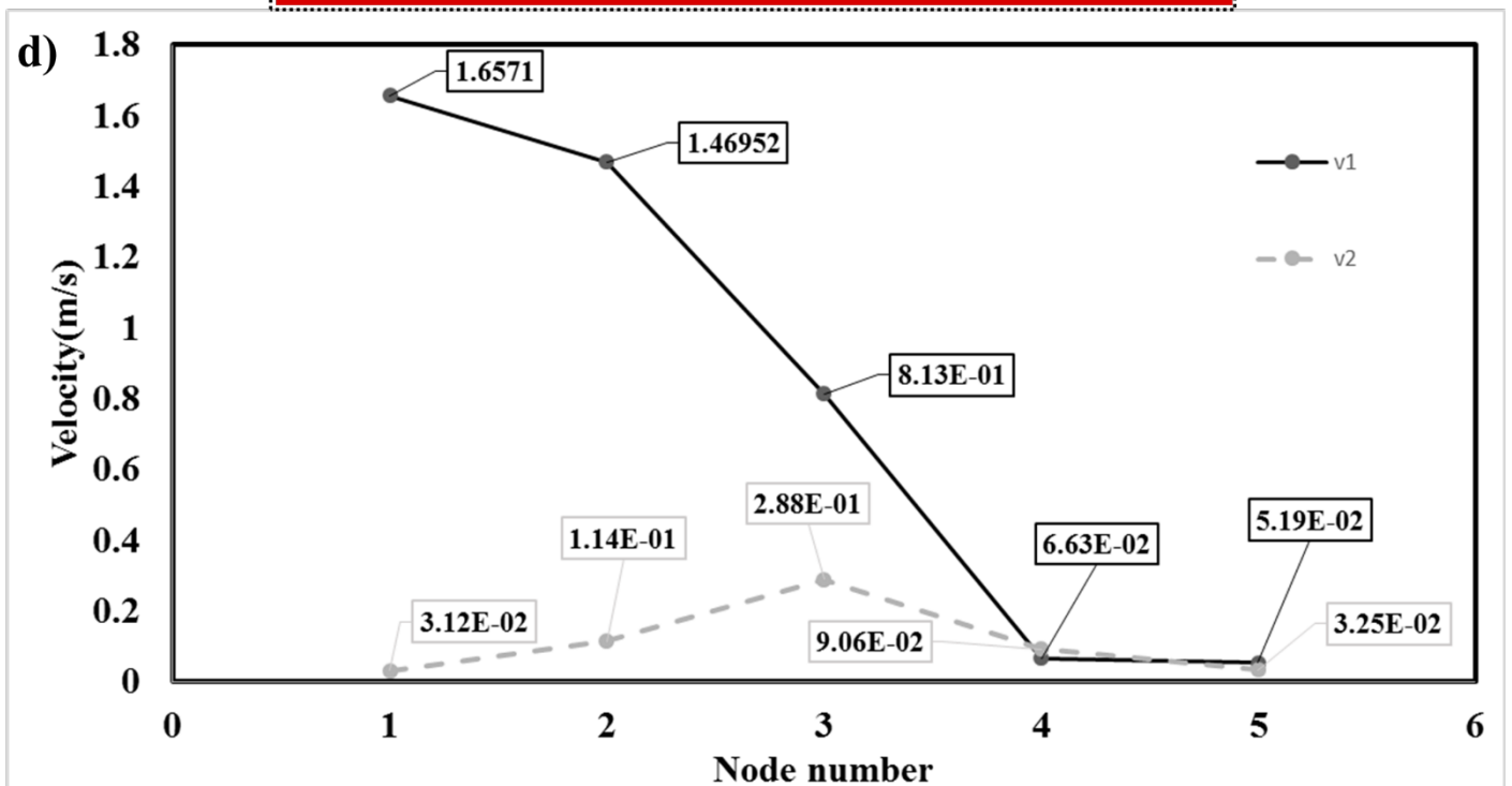
Figure 8. a) Velocity distribution for a rounded tool edge; b) velocity distribution for tool with DMC - Case 4 ( \psi = 15^\circ, \zeta = 15^\circ ); c) arbitrary line AB passing by DMC; c) velocity magnitude of v_1 and v_2 along line
