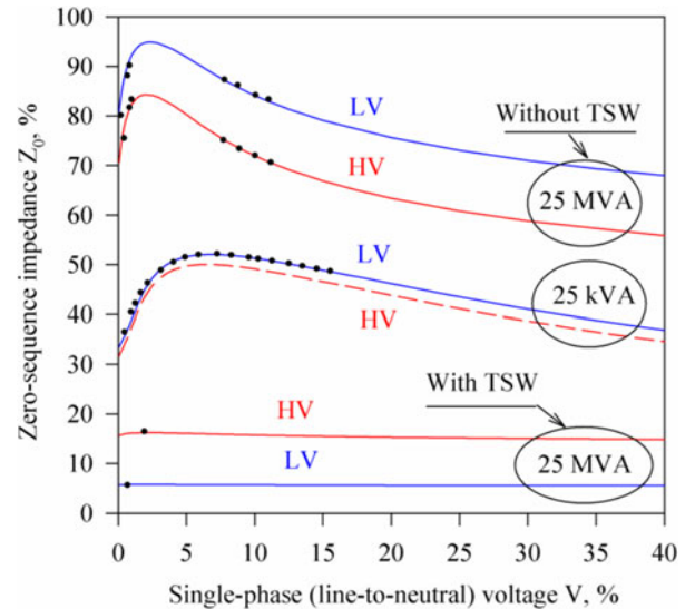
Fig. 4. Variation of the zero-sequence impedance of two core-type transformers with respect to the terminal voltage. Results derive from measurements are represented by dots and those from EMTF simulations with lines [36]. TSW = Tertiary Stabilizing Winding.
