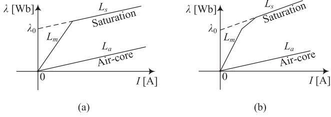
Fig. 2. Comparison of the air-core and terminal saturation inductance: (a) case where the slopes are equal; (b) case where the slopes are different.
